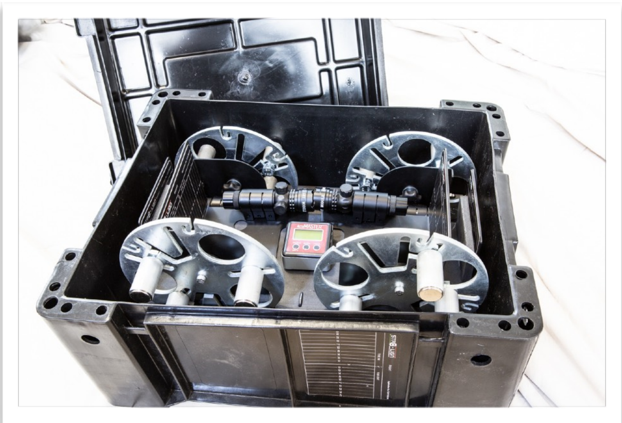
STR8-LIGN TARGET HEAD IN OPERATION - COMPLETE STR8-LIGN UNIT
